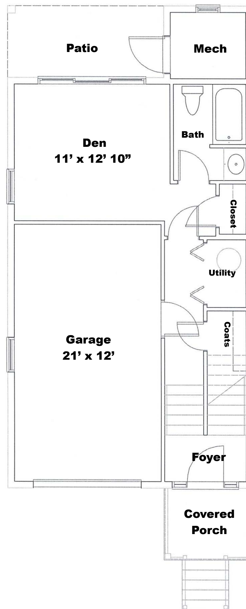
End Unit
